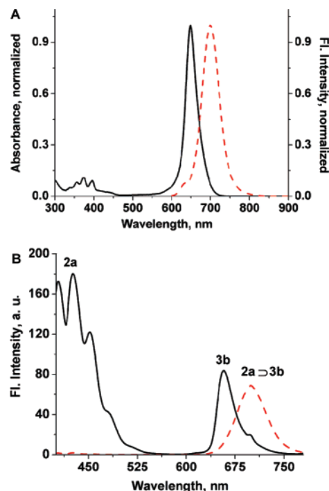
Figure 2. (A) Absorption (black full line) and fluorescence emission (red dashed line, ex: 580 nm) spectra for rotaxane 2a ⊃ 3b in chloroform. (B) Fluorescence emission spectra (ex: 350 nm) for an equimolar mixture of 2a and 3b (both 5 \mu\text{M} ) (black full line) and a solution of 2a ⊃ 3b (red dashed line) in chloroform.
